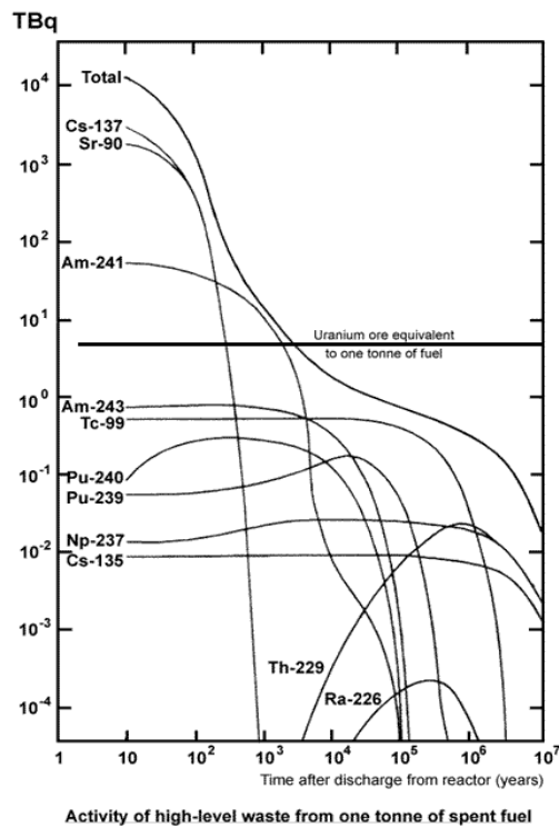
Figure 8. Radioactive Decay of Typical Spent Fuel
